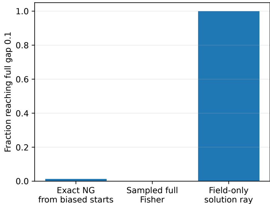
Chain optimization versus representability
