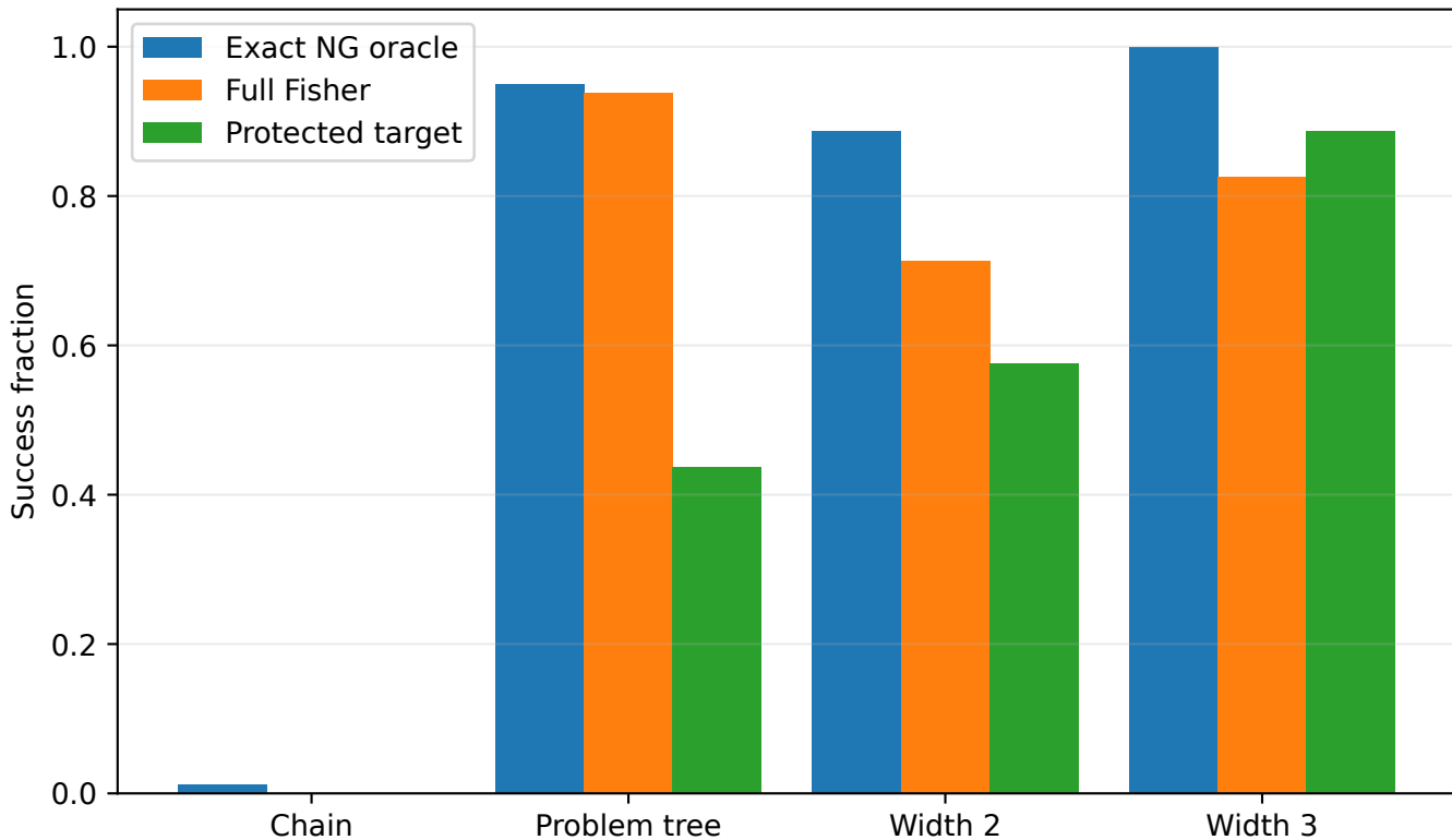
Exact geometric ceiling and finite-sample gap
