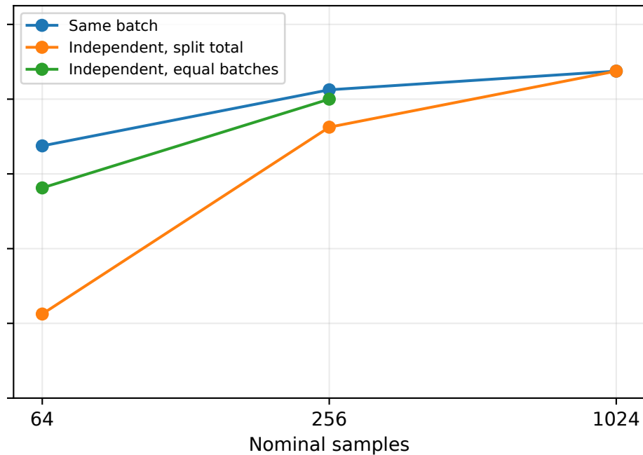
Width-3 sample scaling
