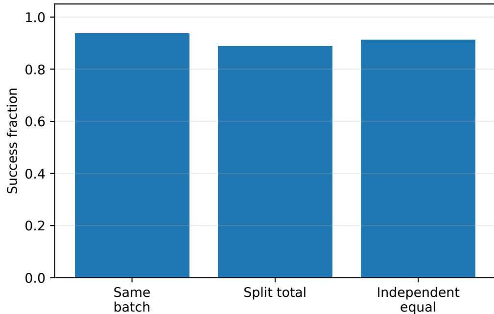
Problem tree, nominal budget 256
