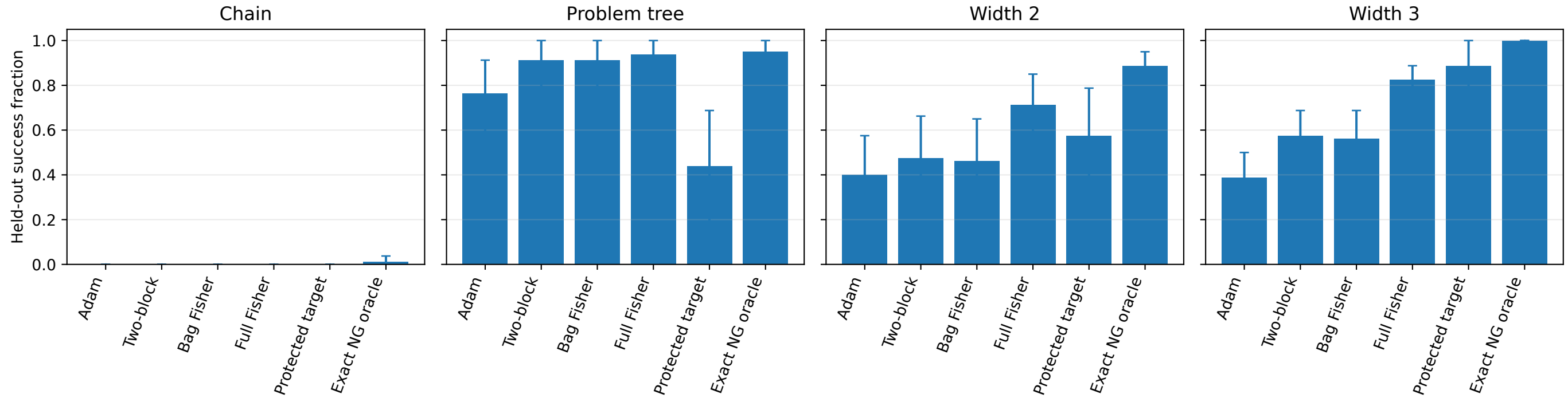
Partial alignment: 256-sample methods versus exact natural-gradient oracle
