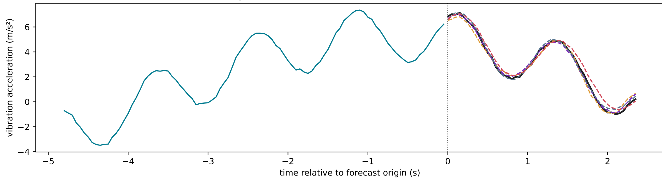
largest combined-model loss: Station 4, Product B
