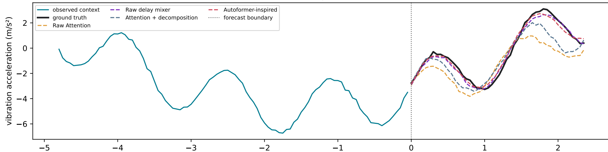
largest combined-model loss: Station 4, Product B
