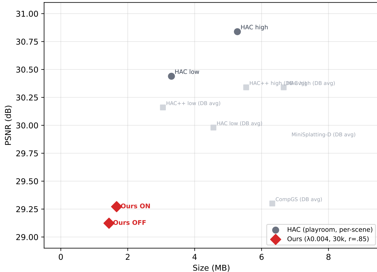
Deep Blending: playroom — per-scene comparison (grey squares = survey DB dataset-average, reference only)
