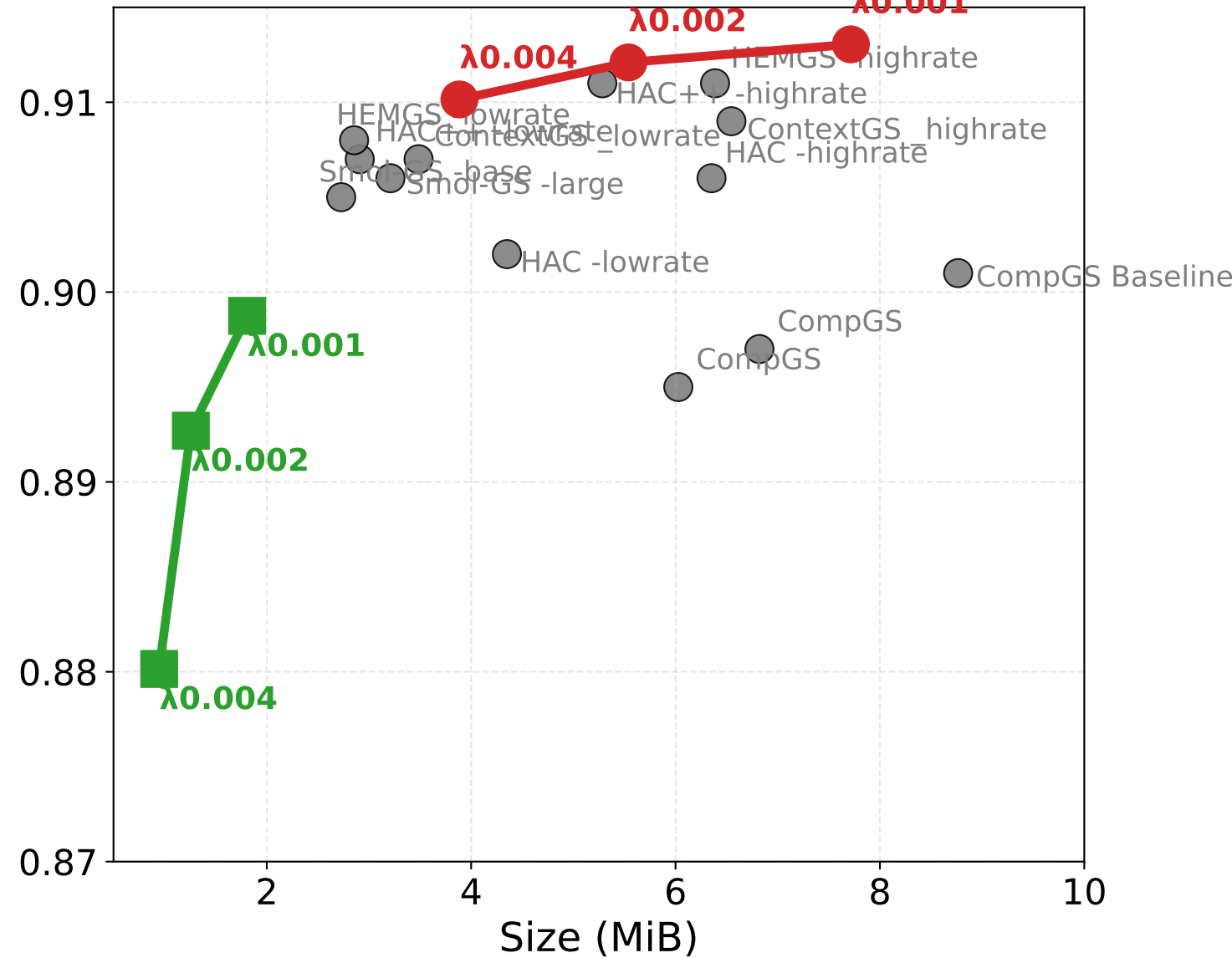
DB RD: SSIM vs Size
