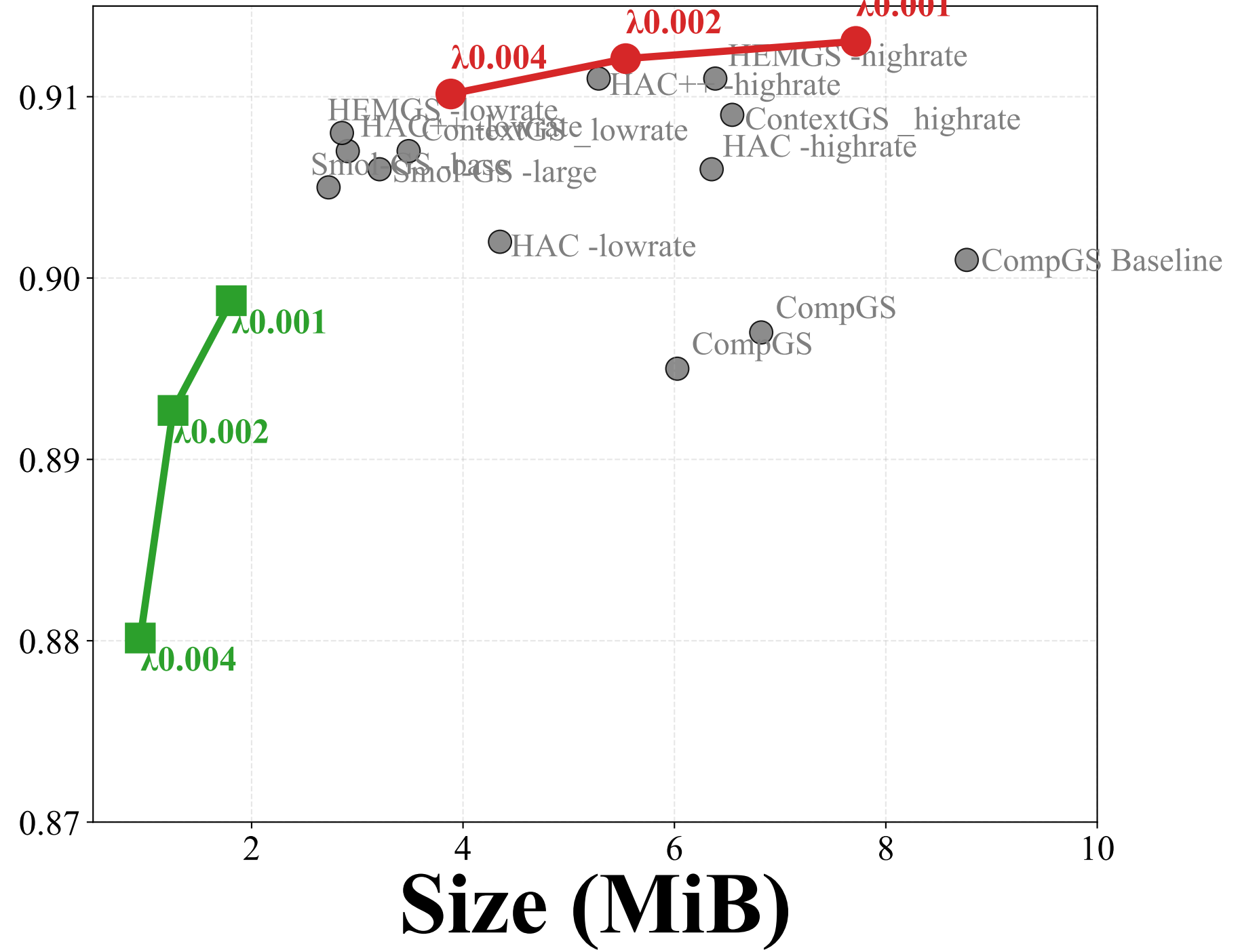
DB RD: SSIM vs Size
