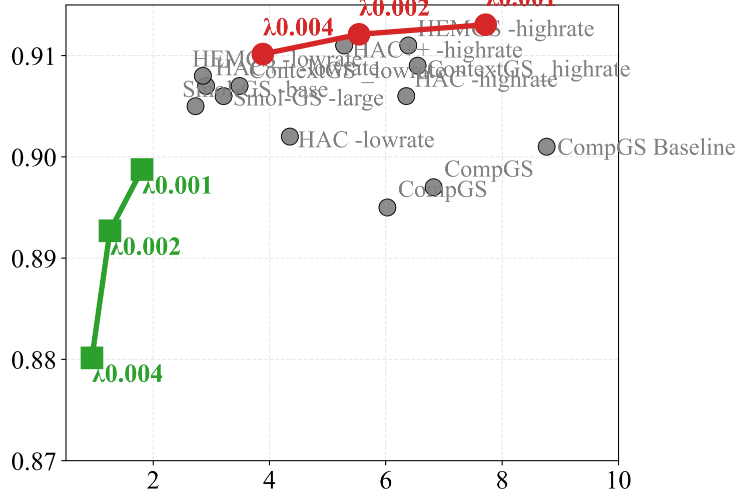
DB RD: SSIM vs Size
