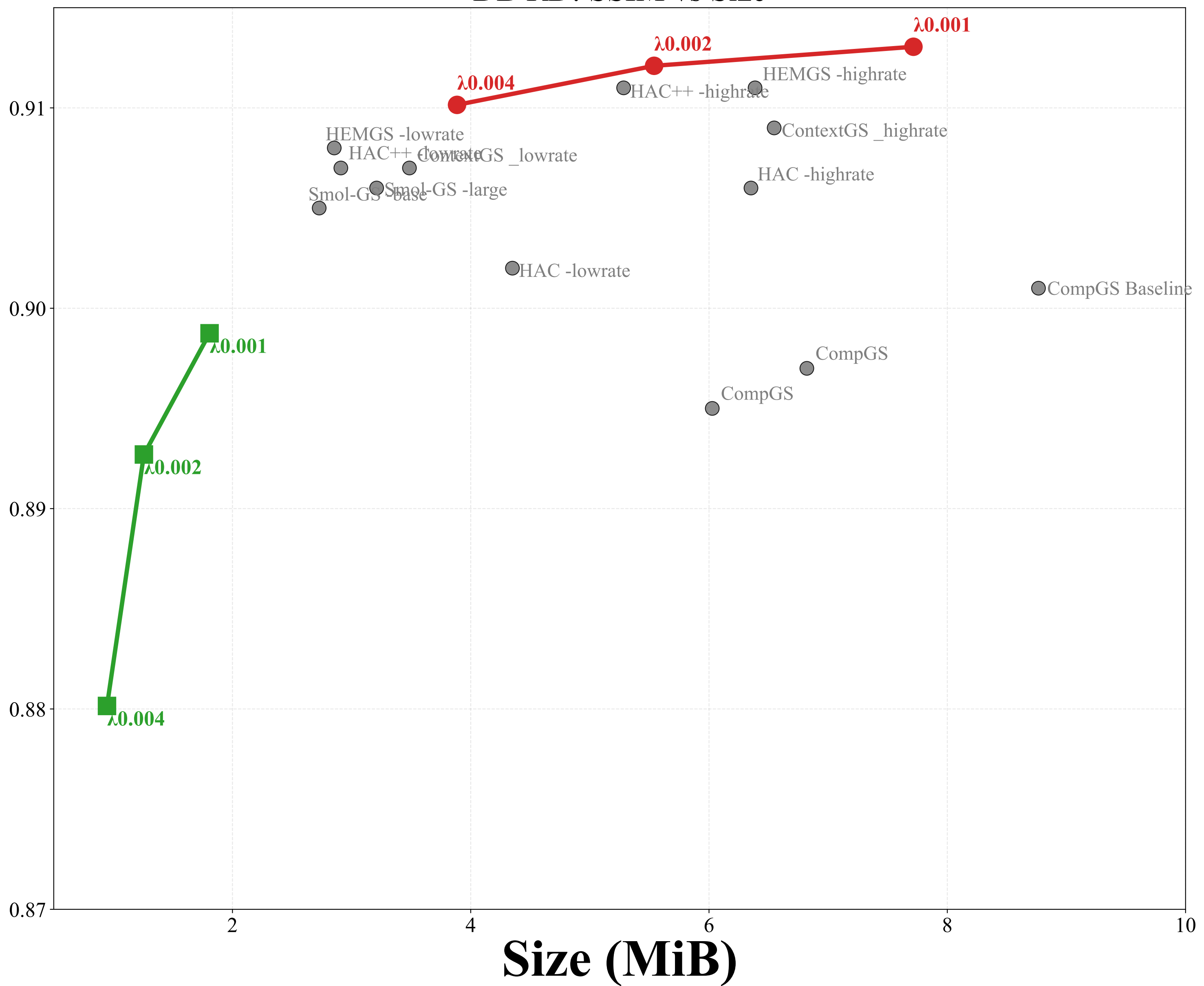
DB RD: SSIM vs Size
