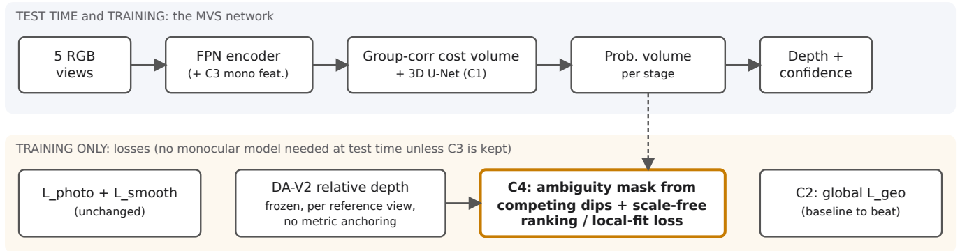
Figure 3. Proposed system. C4 (orange outline) reads the network's own probability volume to find tied hypotheses and uses the monocular model only to rank them.
