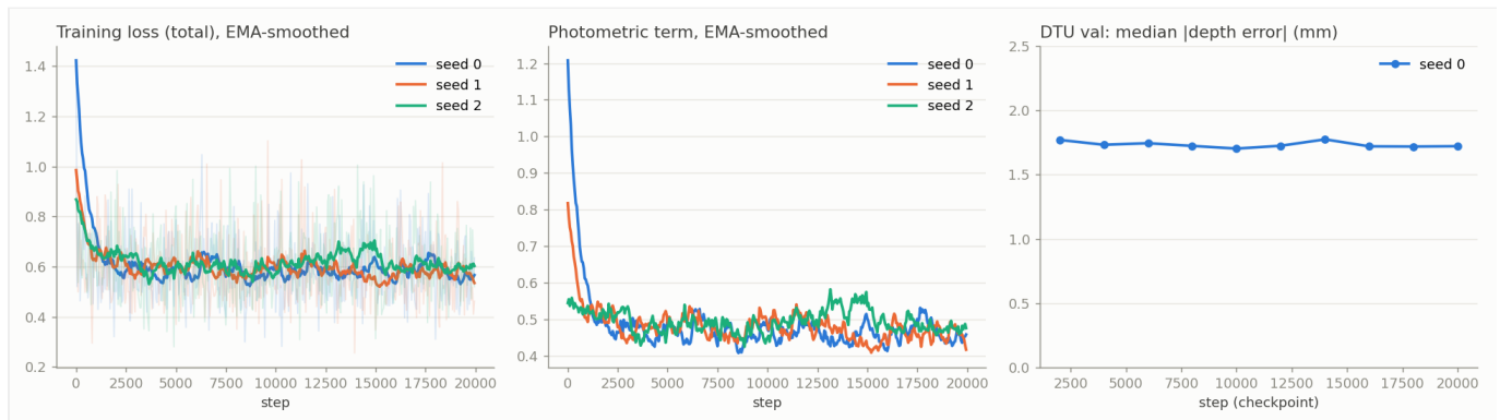
Figure 5. Training curves of the pre-fix A0 base phase (runs/A0_baseline/convergence.png, 3 seeds, 20k steps, constant lr 1e-3). Loss and DTU-val median depth error (~1.72 mm) are flat from ~2k steps. This plateau motivated the CL-MVSNet-recipe fine-tune (phase 2), which gave only ~5%.
