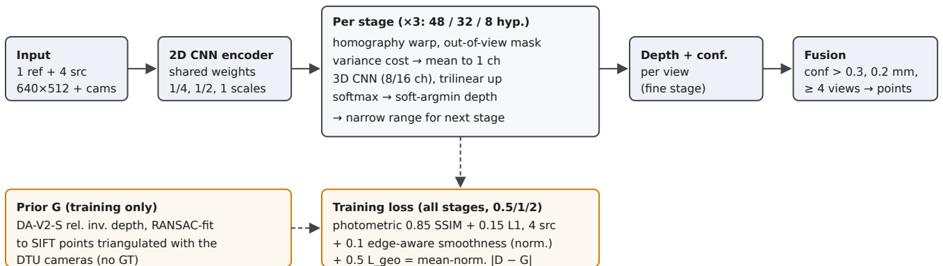
Figure 3. Block diagram of the A0f baseline (Stage 0, frozen).
