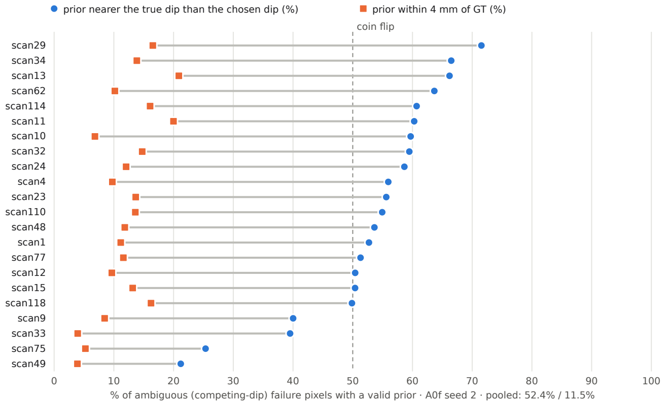
Figure 7. Per-scan prior quality at the failure pixels that matter (ambiguous pixels: the cost curve has competing dips), A0f seed 2, from runs/prior_vs_dips/A0f_seed2.json. Blue = how often the prior is nearer the true dip than the chosen one; orange = how often it is within 4 mm of GT. Pooled over 22 scans: 52.4% and 11.5%. Most scans sit near the 50% coin-flip line.
