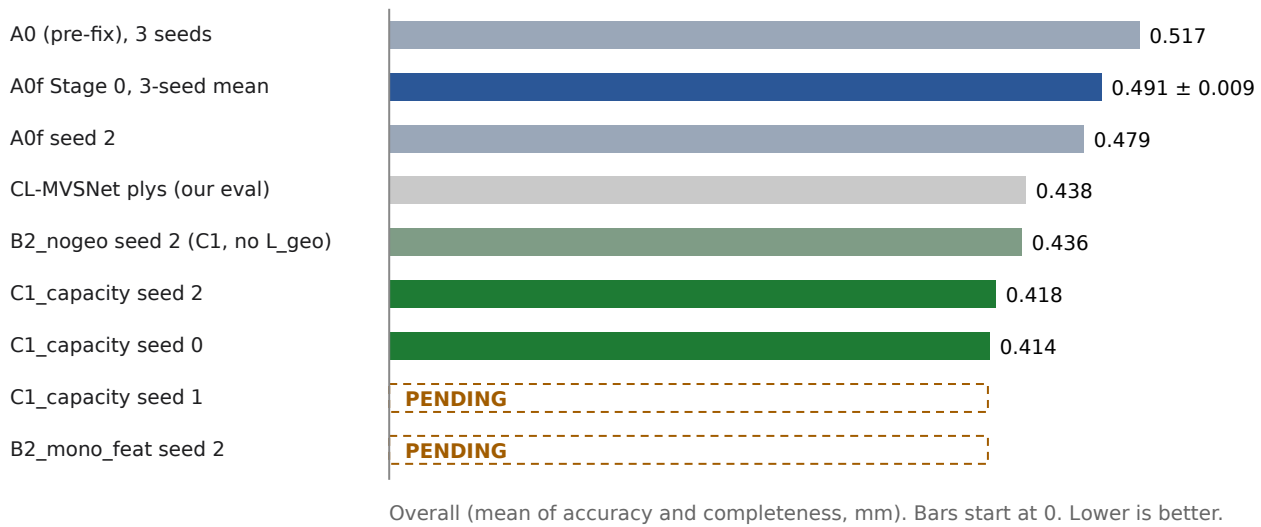
Figure 2. Headline fused overall scores (mm, lower is better) under our evaluator, from the run JSONs. Dashed bars are PENDING.
