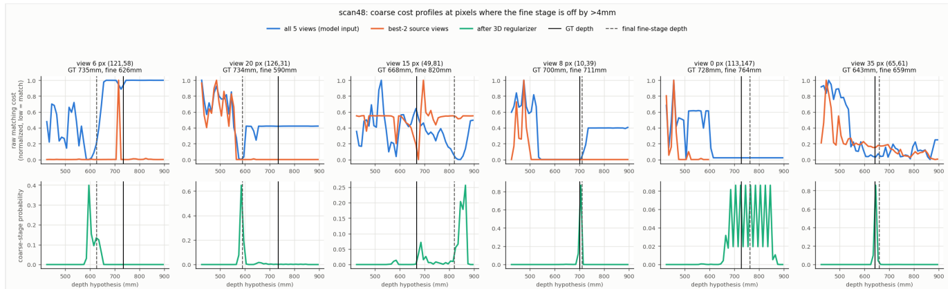
Figure 6. Raw cost profiles at scan48 pixels where the fine stage is off by > 4 mm (runs/A0_finetune_clmvs/seed2/probe/scan48_coarse_profiles.png; the A0 fine-tune checkpoint, the predecessor of A0f). Solid black = GT depth, dashed = predicted. The GT is often a secondary dip ("competing dips") or not a minimum at all, and the 3D regularizer commits to the wrong mode. Image evidence alone cannot decide these pixels.
