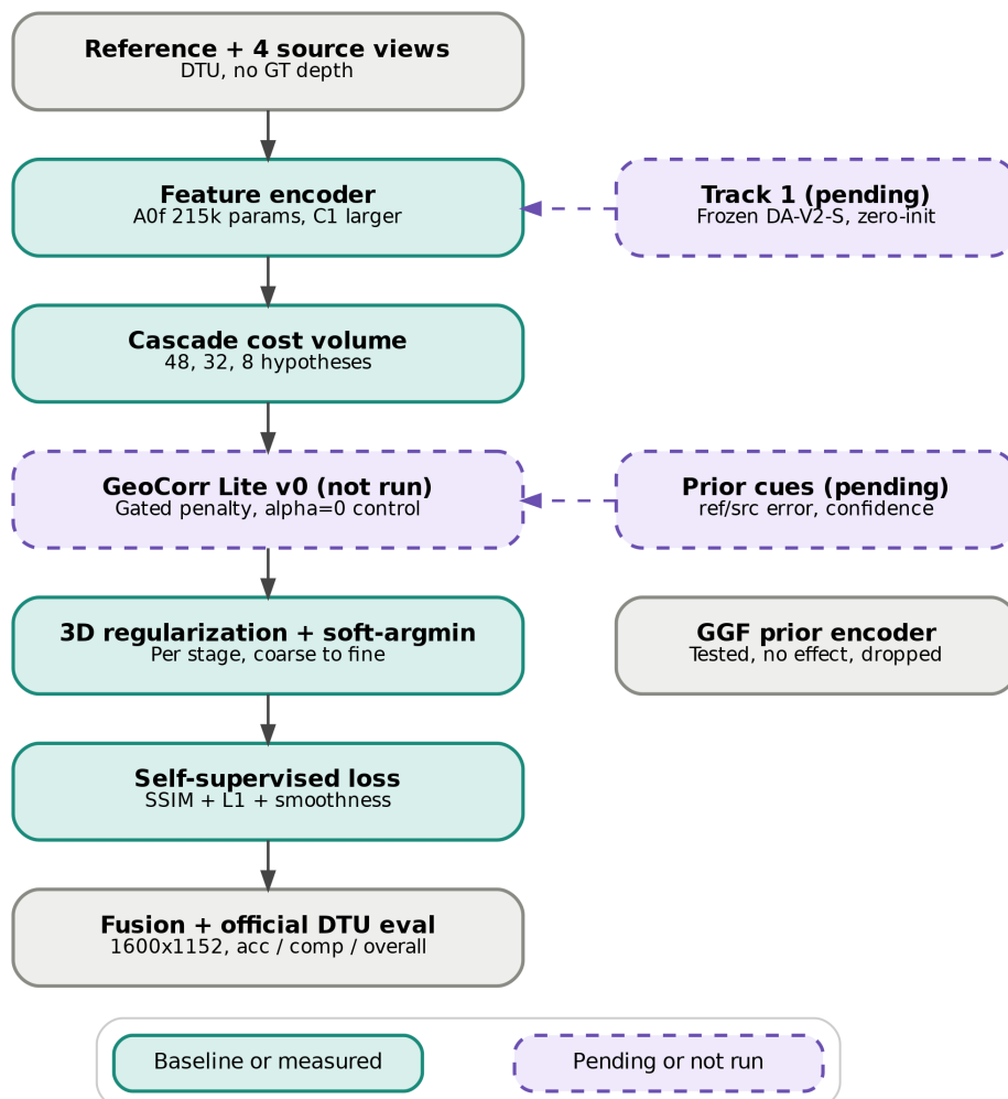
Figure 9. Proposed pipeline with the open work attached (reports/figs/proposal_block_diagram.png, graphviz, 300 dpi; source .dot and .svg alongside). Teal = baseline or measured; purple dashed = pending or not run. The GGF prior encoder is shown without arrows because it was tested and dropped.
