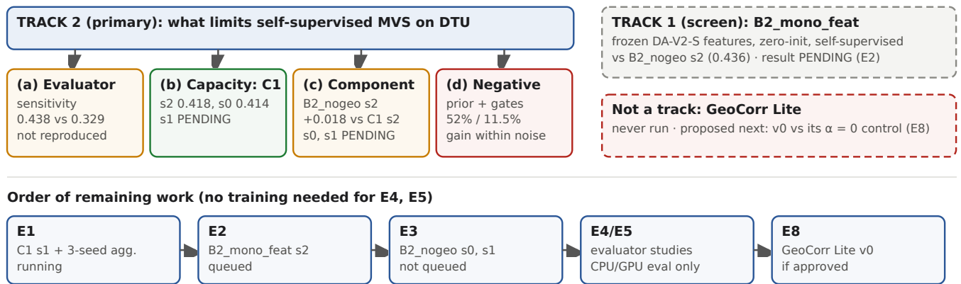
Figure 8. Structure of the revised direction: Track 2 (primary, four findings), Track 1 (screen), GeoCorr Lite (not a track, never run), and the order of the remaining experiments (§6.1).
