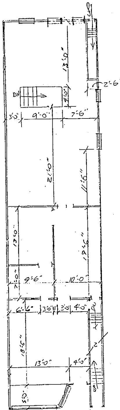
115 W. JACKSON FIRST FLOOR
