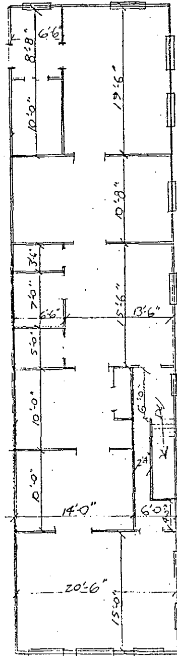
115 W JACKSON SECOND FLOOR
