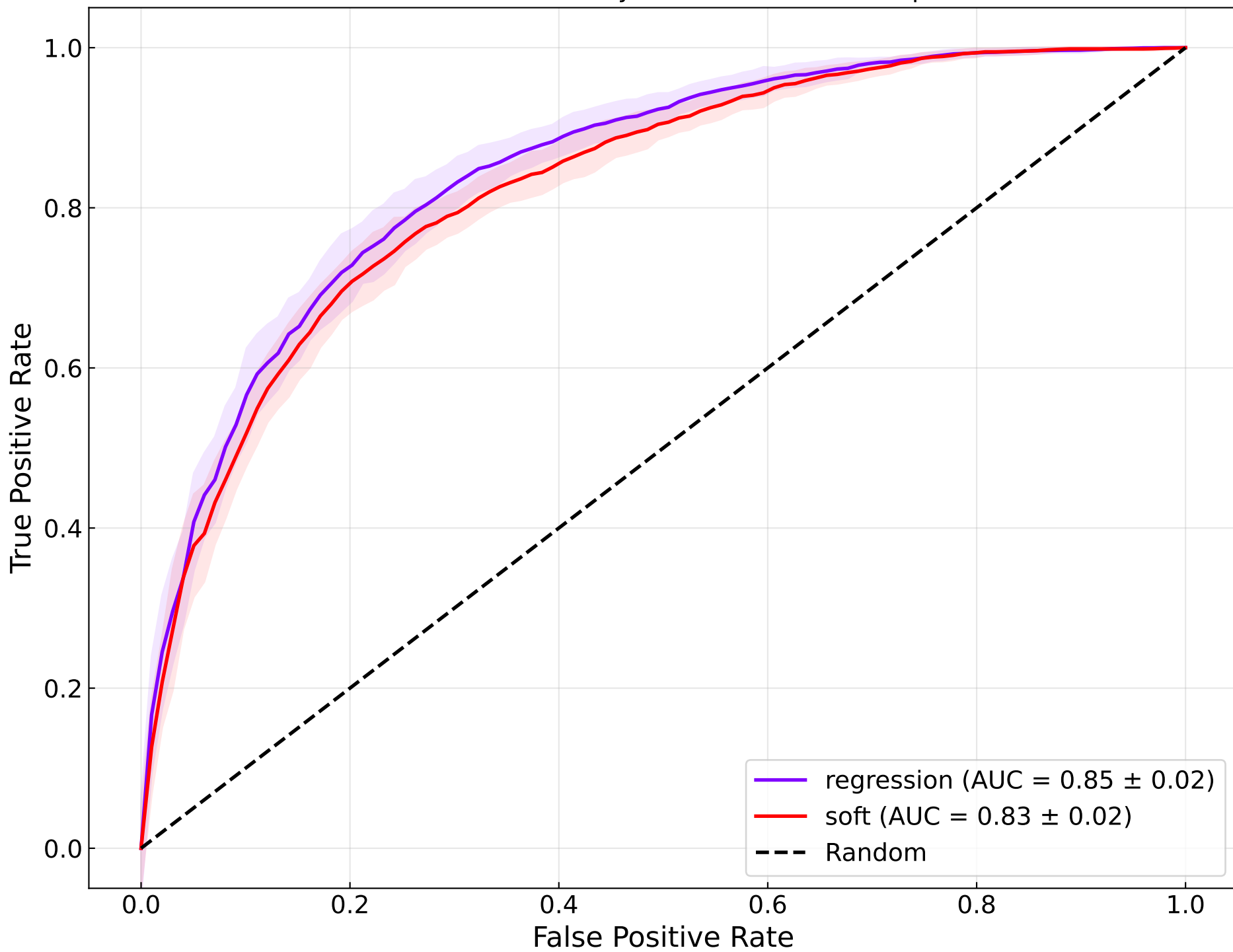
Mean ROC curves by GCN model, random split
