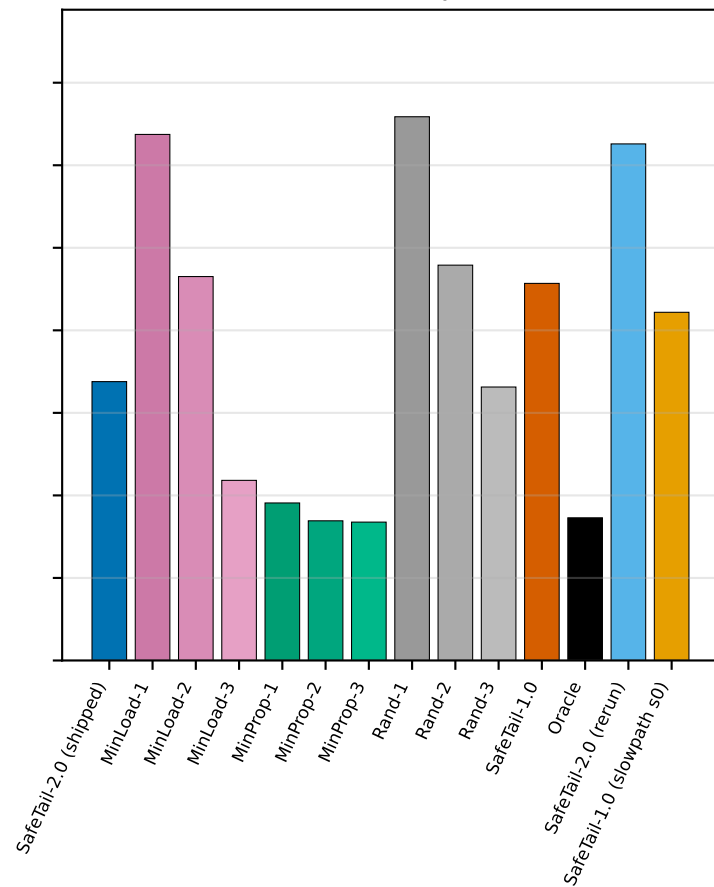
Predict (p)
