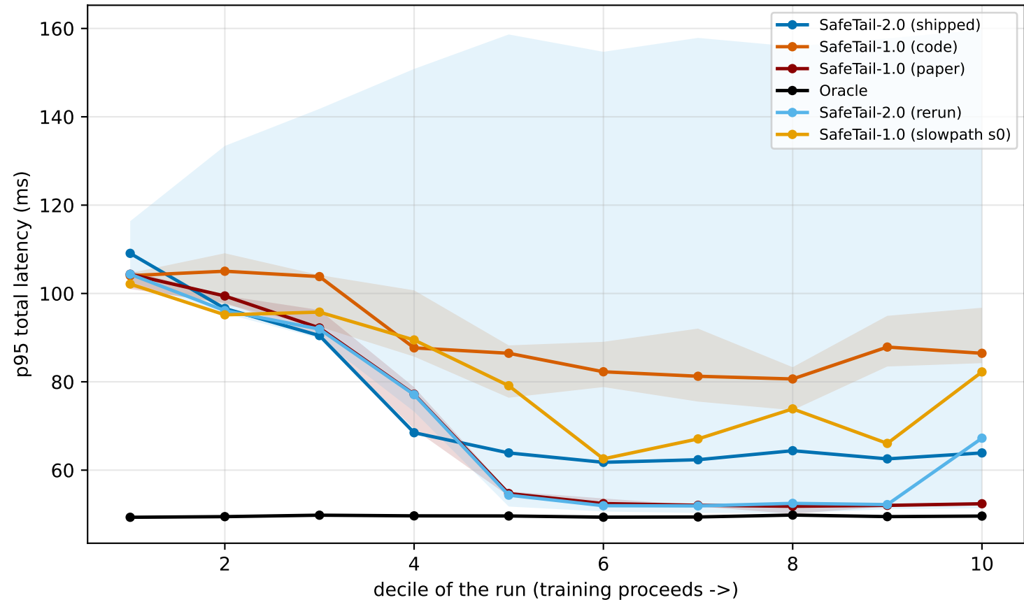
Convergence: p95 within each decile (line = median across seeds, band = min/max)
