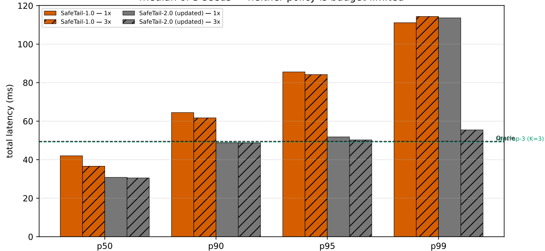
Data budget: 1x vs 3x, CONVERGED phase only (last third of run) median of 3 seeds — neither policy is budget-limited
