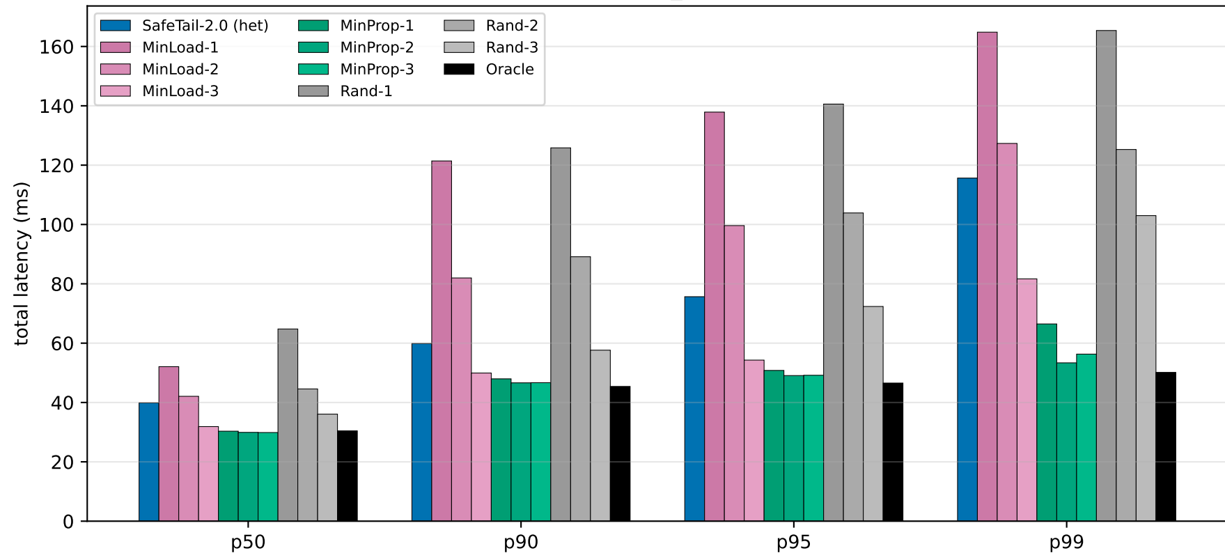
Tail latency by percentile — total_latency (n=14723 per policy)
