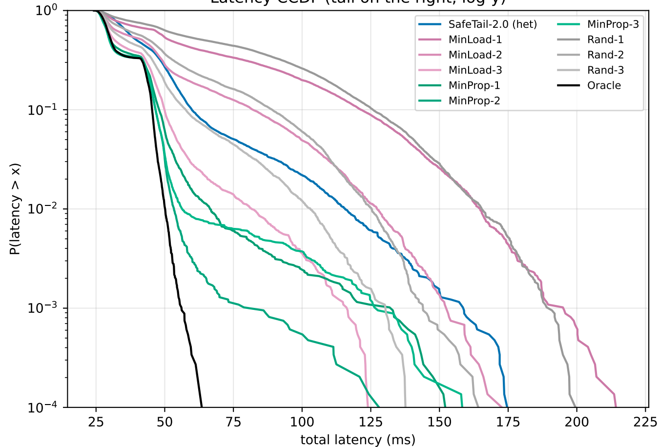
Latency CCDF (tail on the right, log-y)
