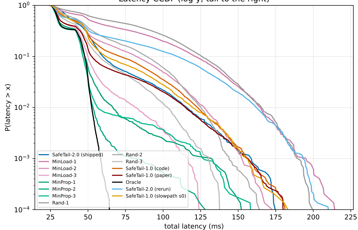
Latency CCDF (log-y; tail to the right)
