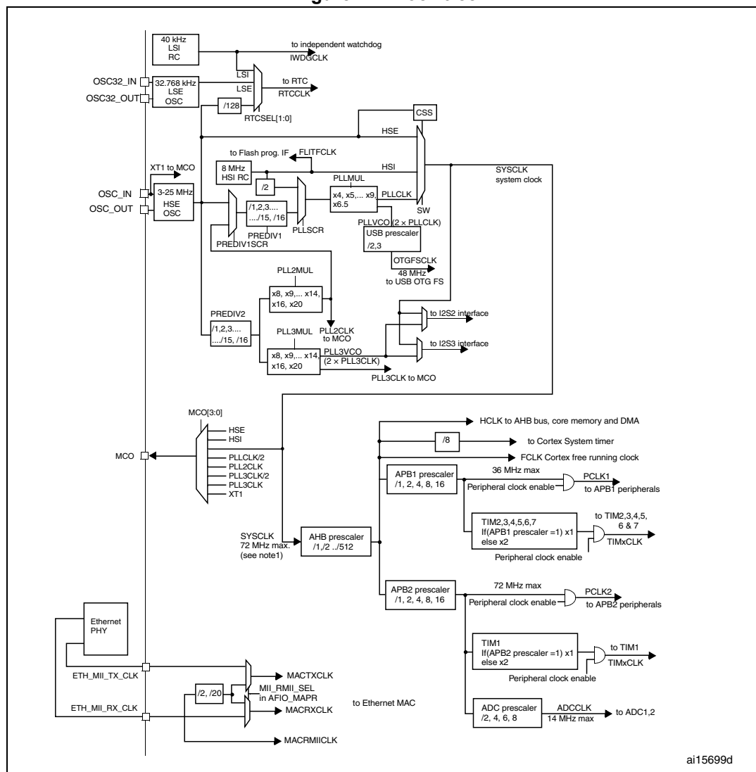
Figure 11. Clock tree
