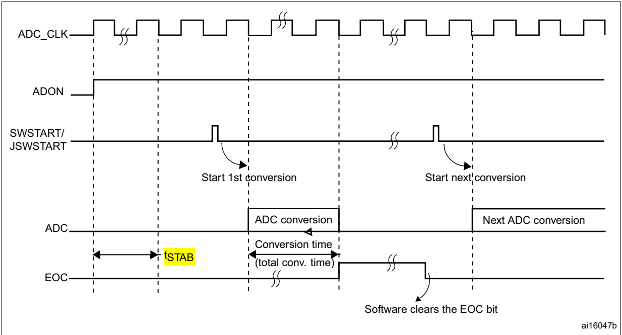
Figure 23. Timing diagram
