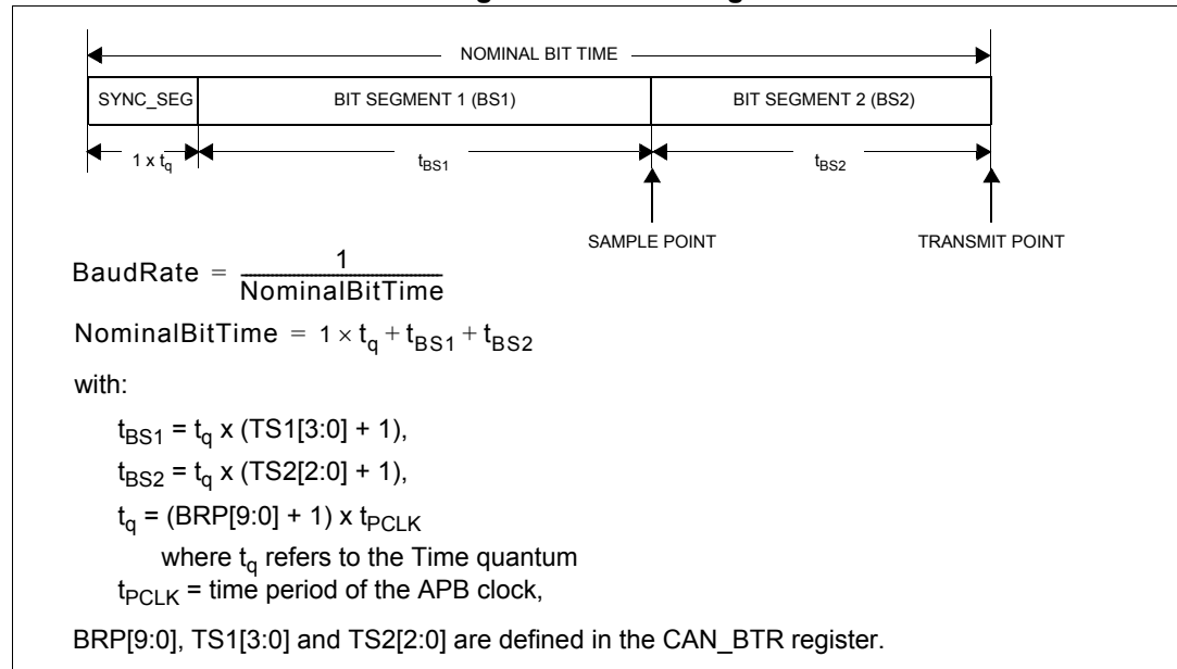
Figure 234. Bit timing
