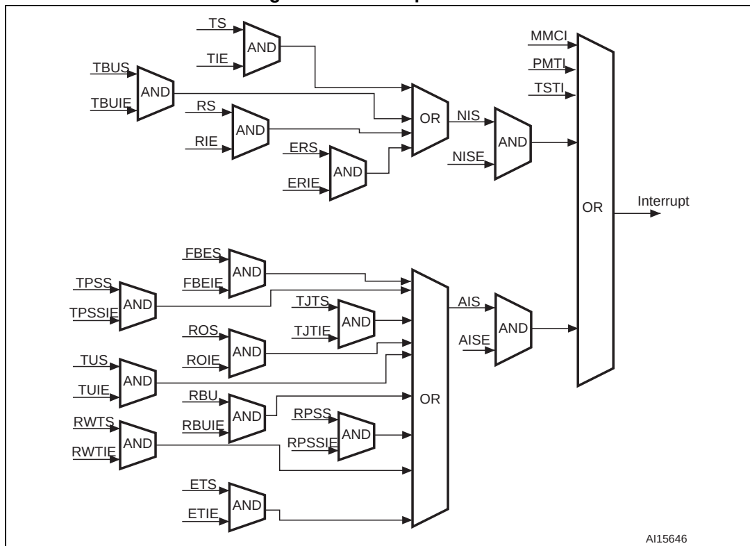
Figure 359. Interrupt scheme
