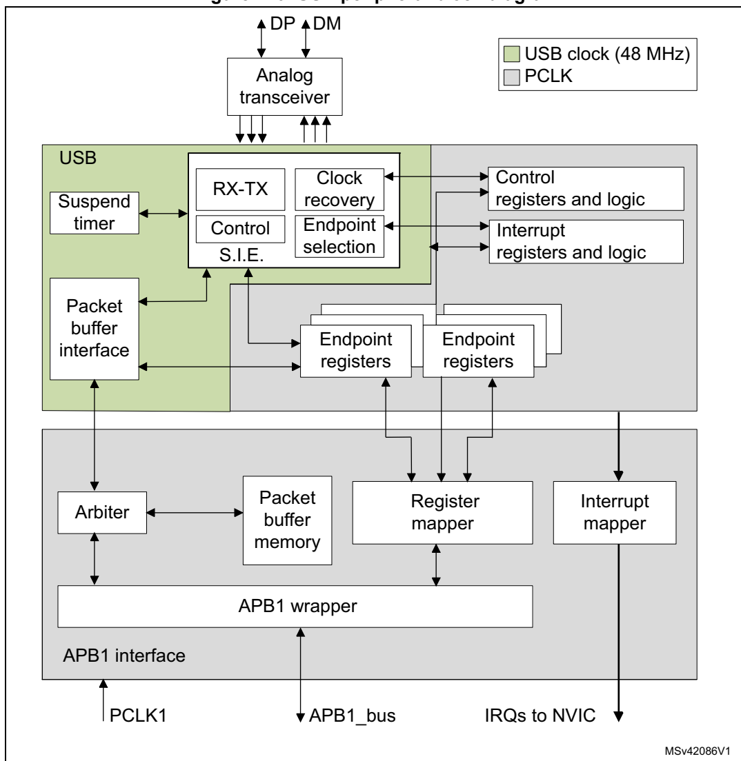
Figure 220. USB peripheral block diagram
