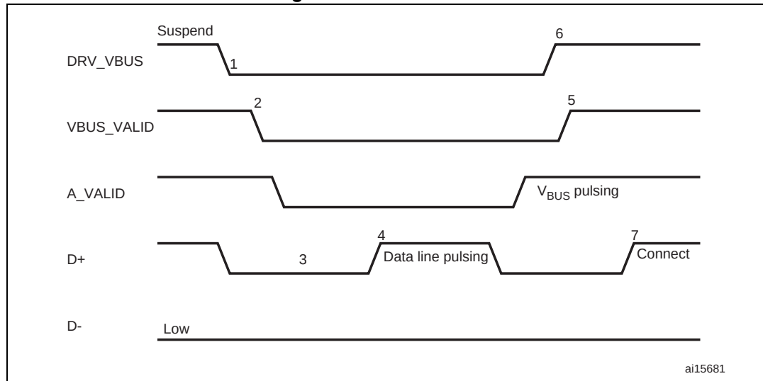
Figure 323. A-device SRP
