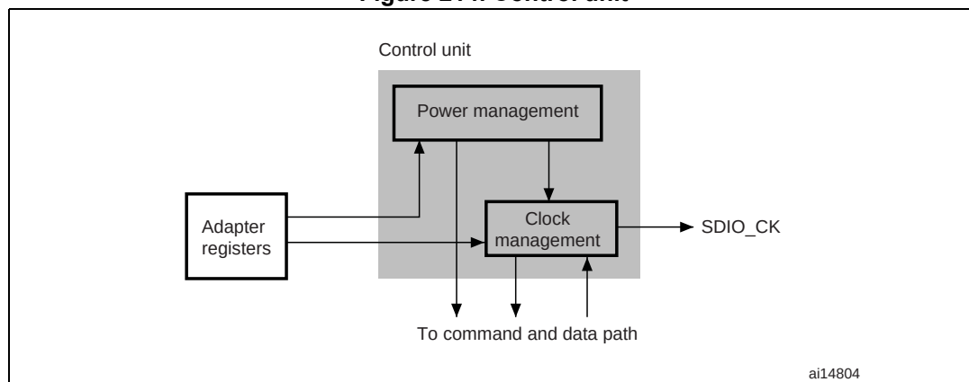
Figure 214. Control unit
