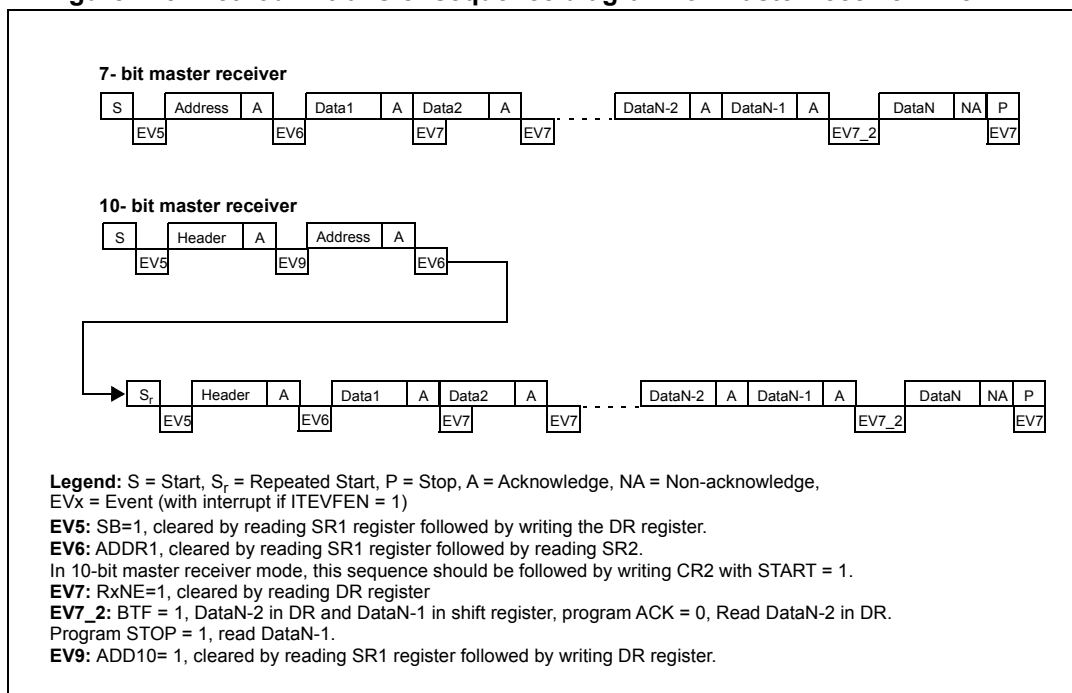
Figure 275. Method 2: transfer sequence diagram for master receiver when N&gt;2
