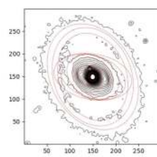
Fig. 8. The final developed outer-ring galaxy analysis sequence. Step 1: Get the code and data from our GitHub as the data collection step, Step 2: Perform descriptive statistics as the data exploration step and check galaxy images, Step 3: Remove the background sky brightness and perform smoothing as the data processing step, Step 4: Perform distinction three-factor analysis of outer-ring galaxy, after performing isoluminant fitting analysis through elliptic geometry calculation as the data analysis step (If there is stars or is complicated inside, additional complementing methods are carried out).
