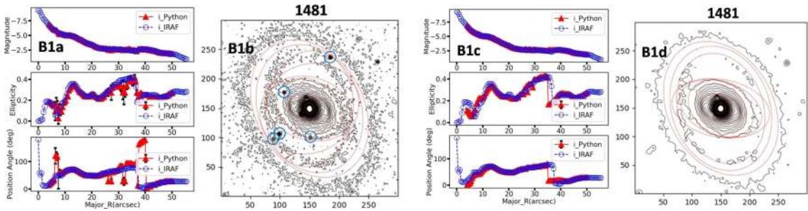
Fig 4. B1a: Mu, Ep, PA of i filter of 1481 outer ring galaxy before complementing, B1b: Distribution of isoluminosity curve at 9 equal intervals of i filter before complementing(dotted line). Symbol small circles indicate removed stars, B1c: Mu, Ep, PA of i filter after complementing, B1d: Distribution of isoluminosity curve at 9 equal intervals of i filter after complementing(dotted line).
