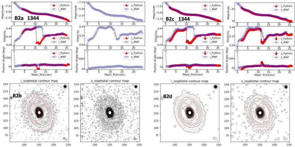
Fig. 5. B2a: Mu, Ep, PA of i, z filter of 1344 outer-ring galaxy before complementing, B2b: Distribution of isoluminosity curve at 9 equal intervals before complementing(dotted line), B2c: Mu, Ep, PA of i, z filter after complementing, B2d: Distribution of isoluminosity curve at 9 equal intervals after complementing(dotted line).
