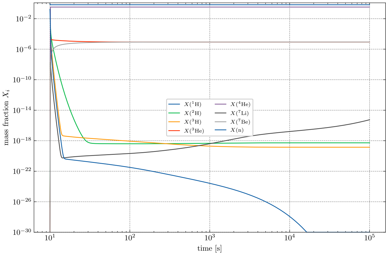
BBN abundances, t_0 = 10 s
