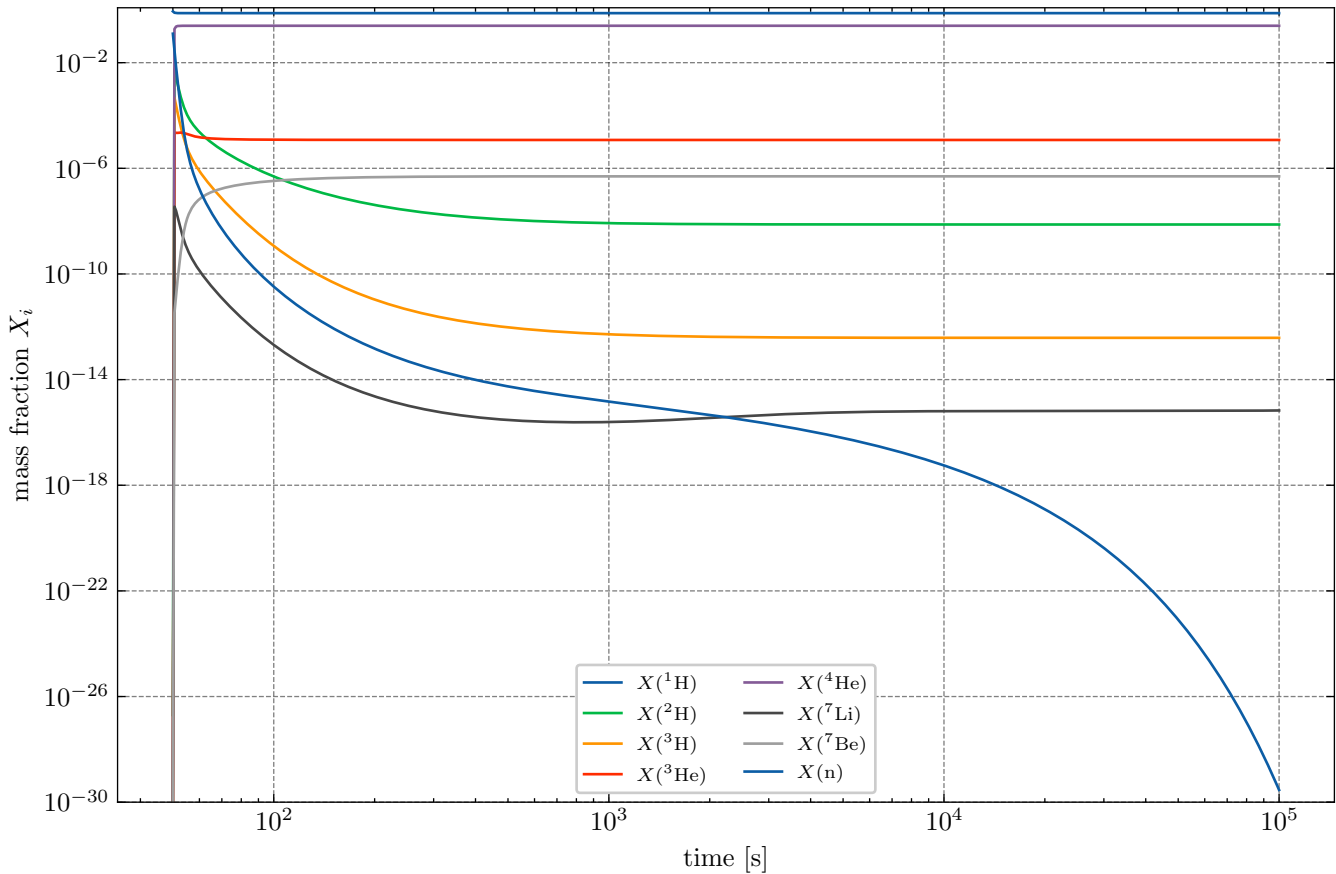
BBN abundances, t_0 = 50 s
