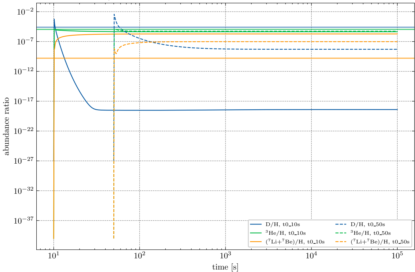
Key BBN abundance ratios: models and observational bands
