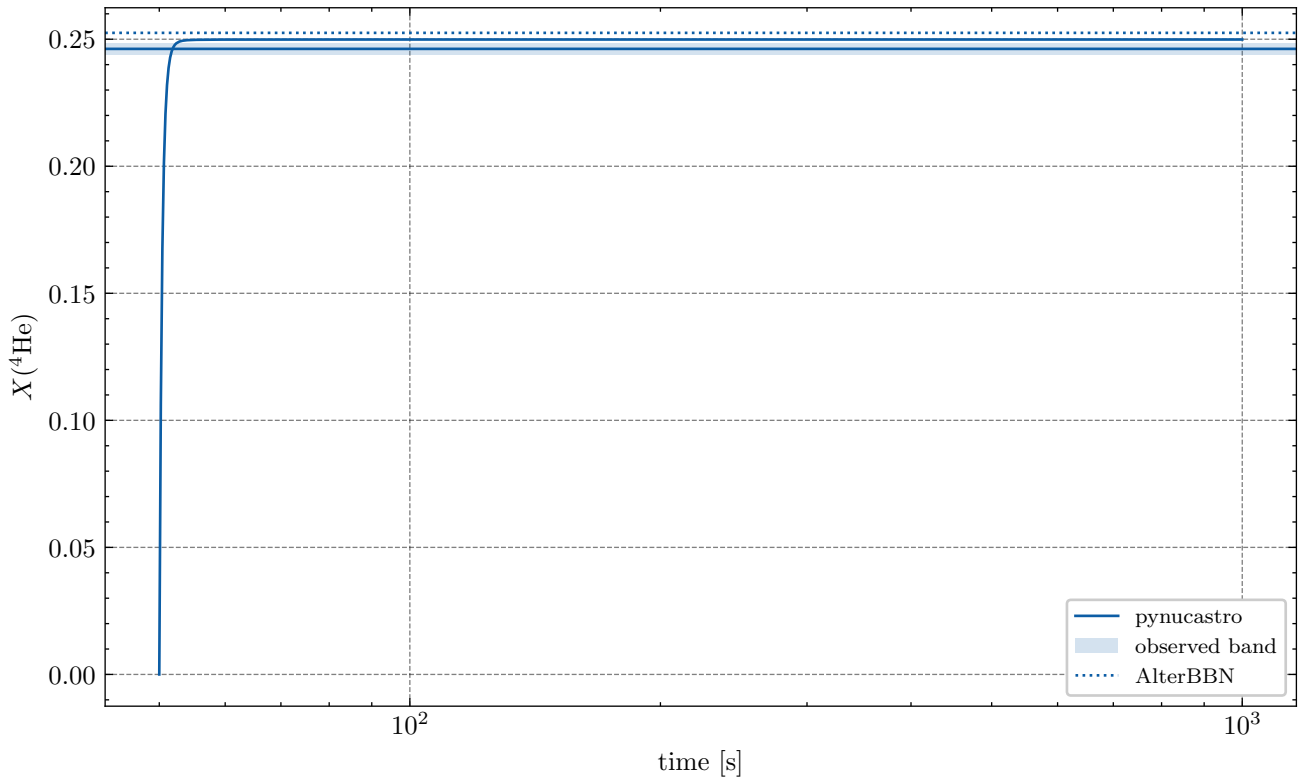
Helium-4 mass fraction
