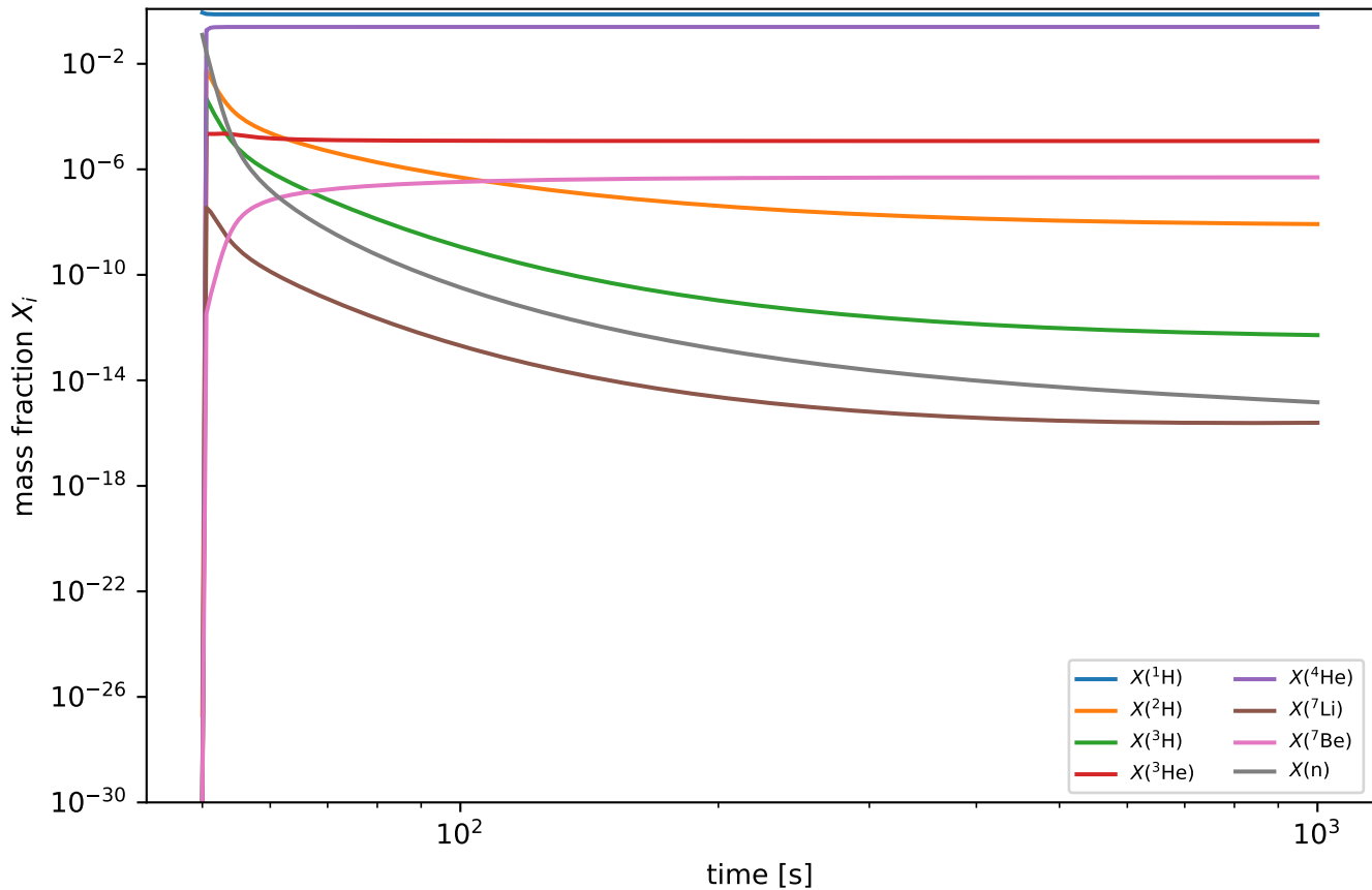
BBN abundances, pynucastro
