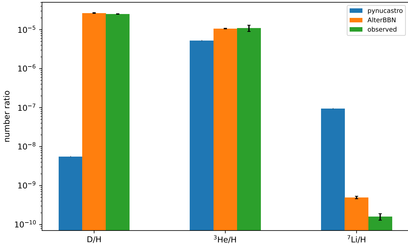
Final BBN benchmark
