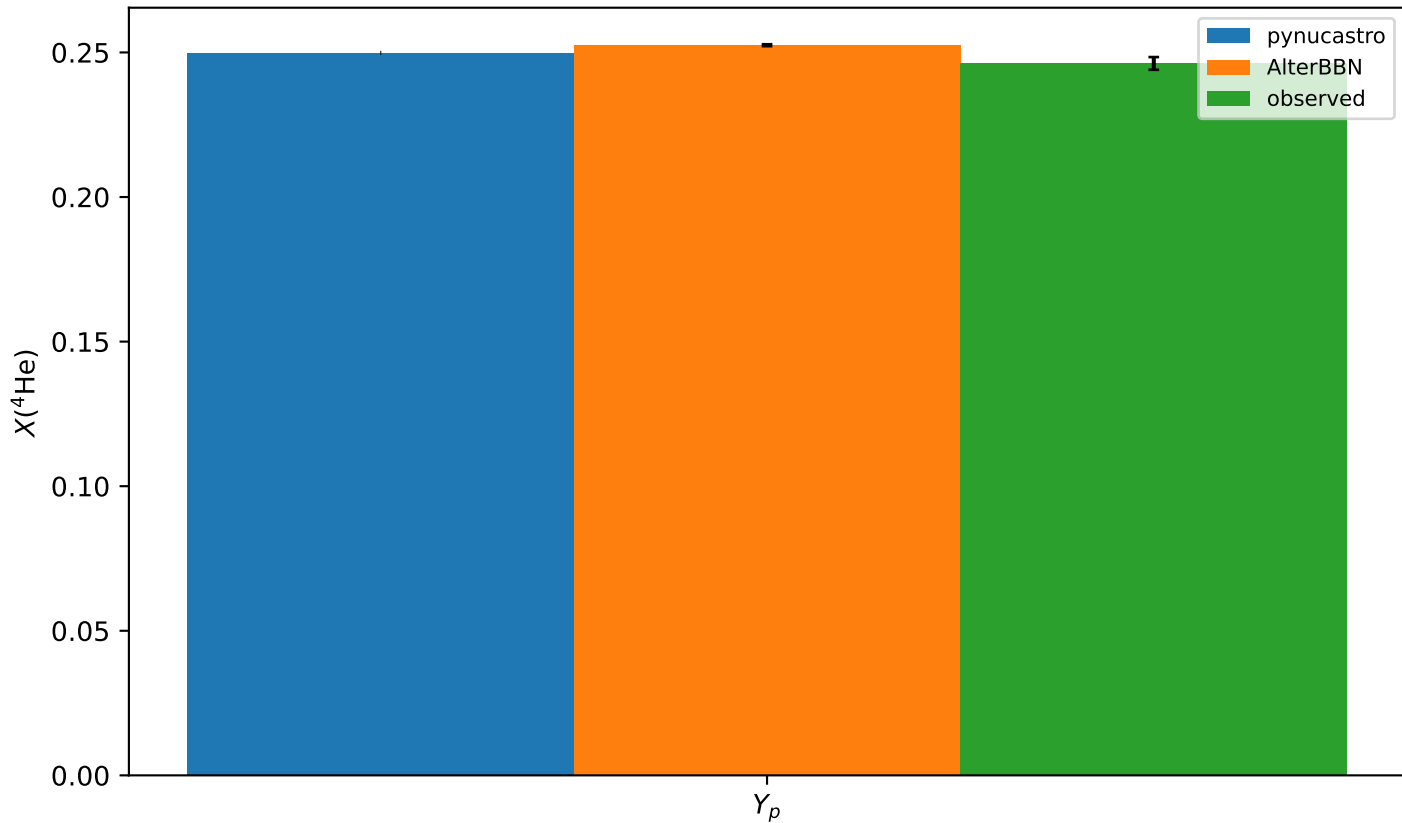
Final helium-4 mass fraction
