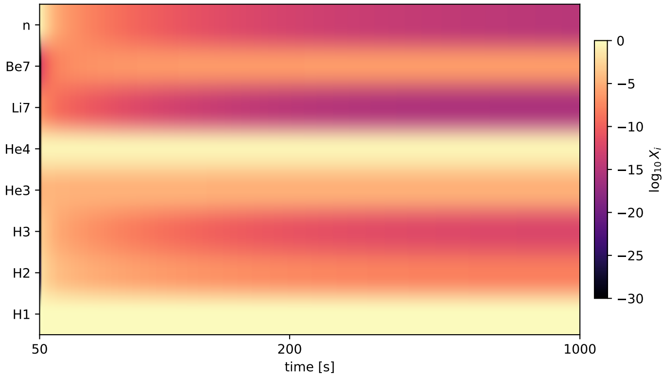
Abundance heatmap, pynucastro
