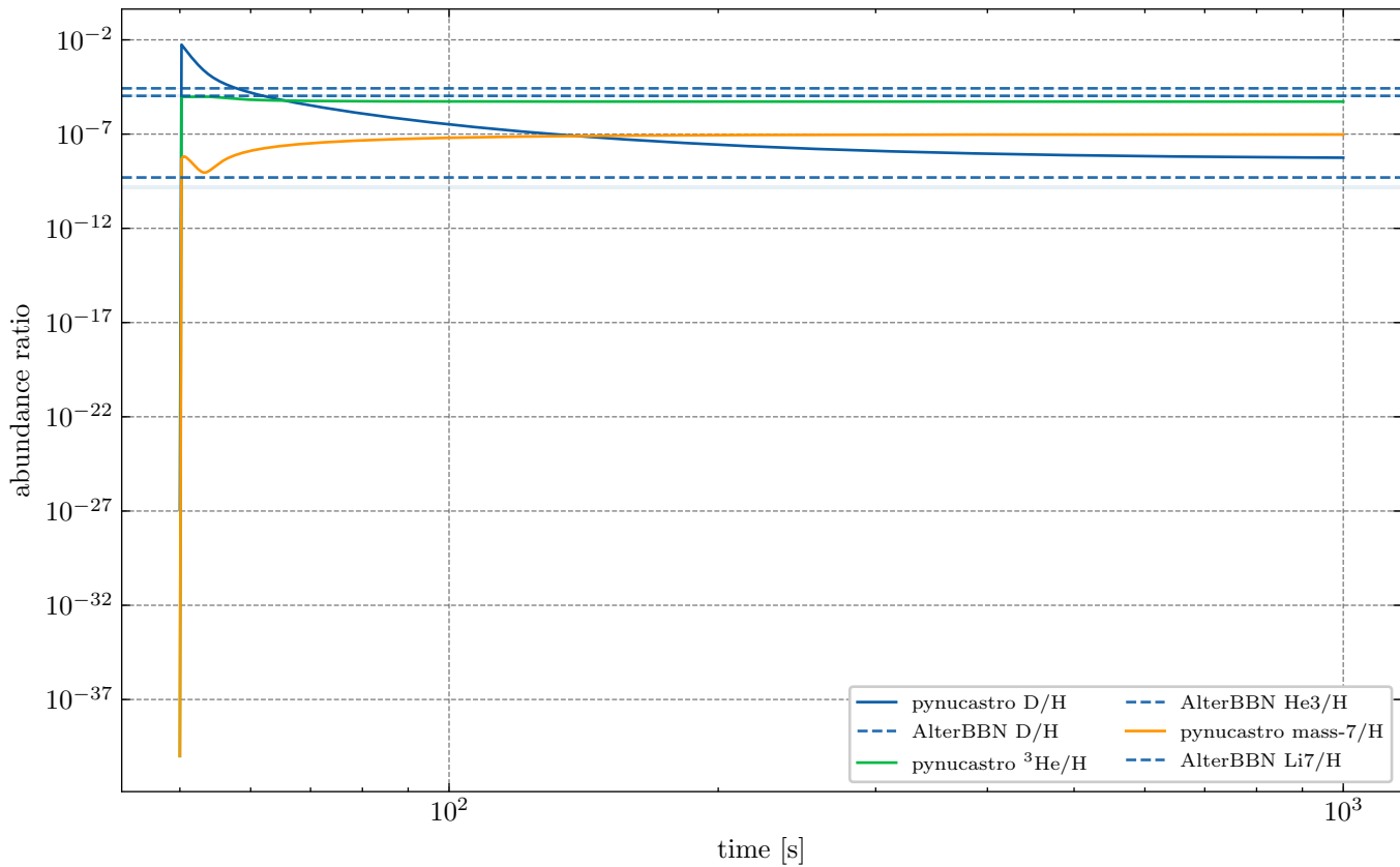
pynucastro evolution vs AlterBBN and observations
