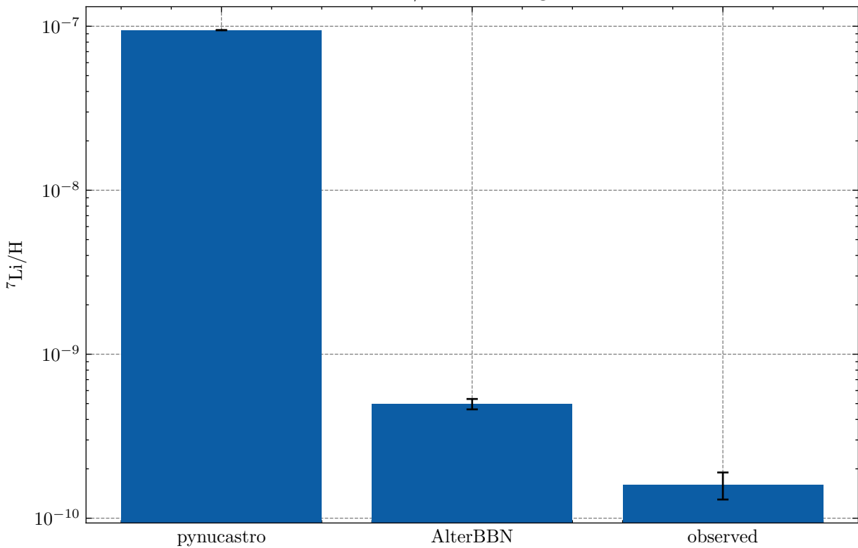
Mass-7 / lithium diagnostic
