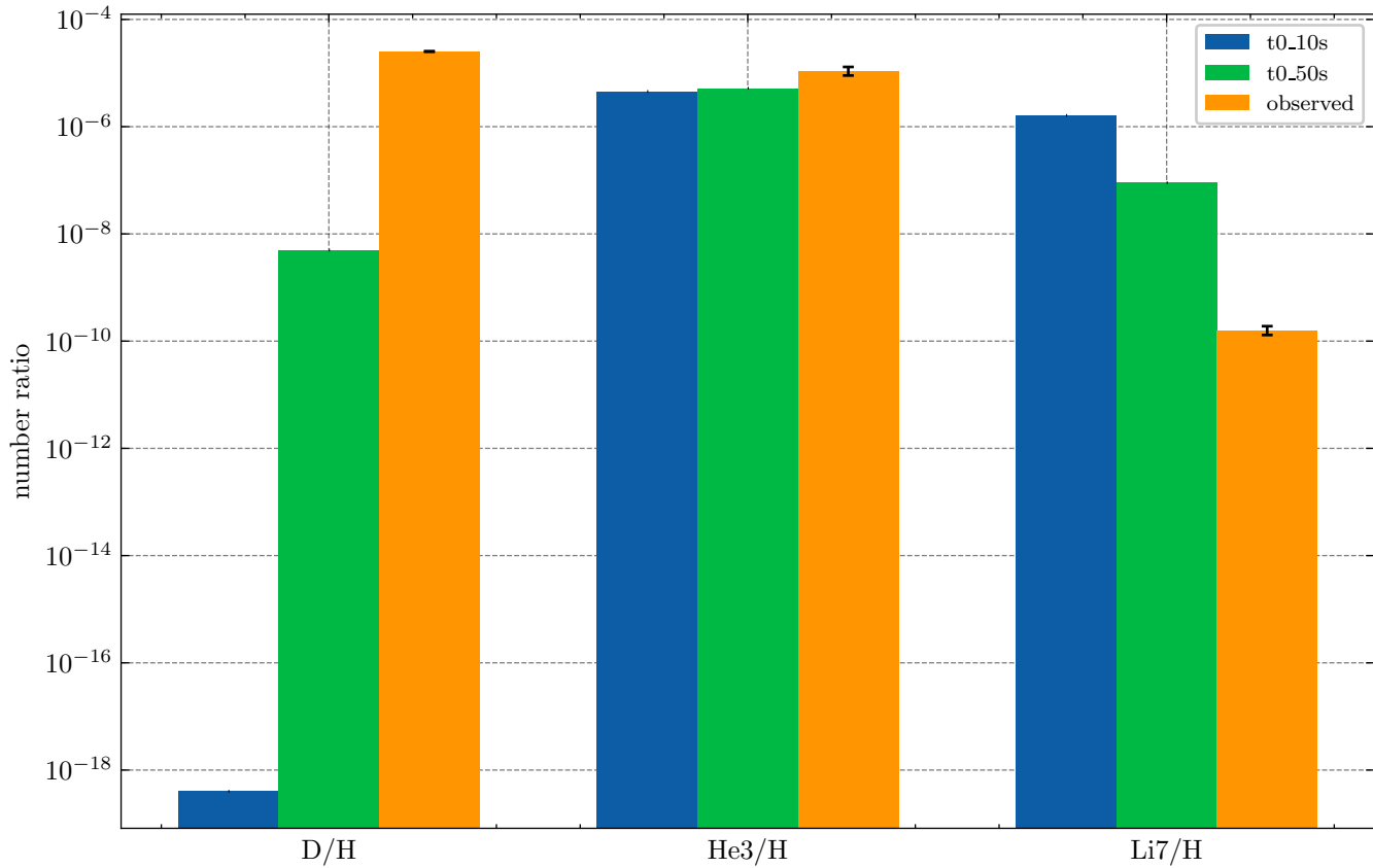
Final abundance ratios: models vs observations
