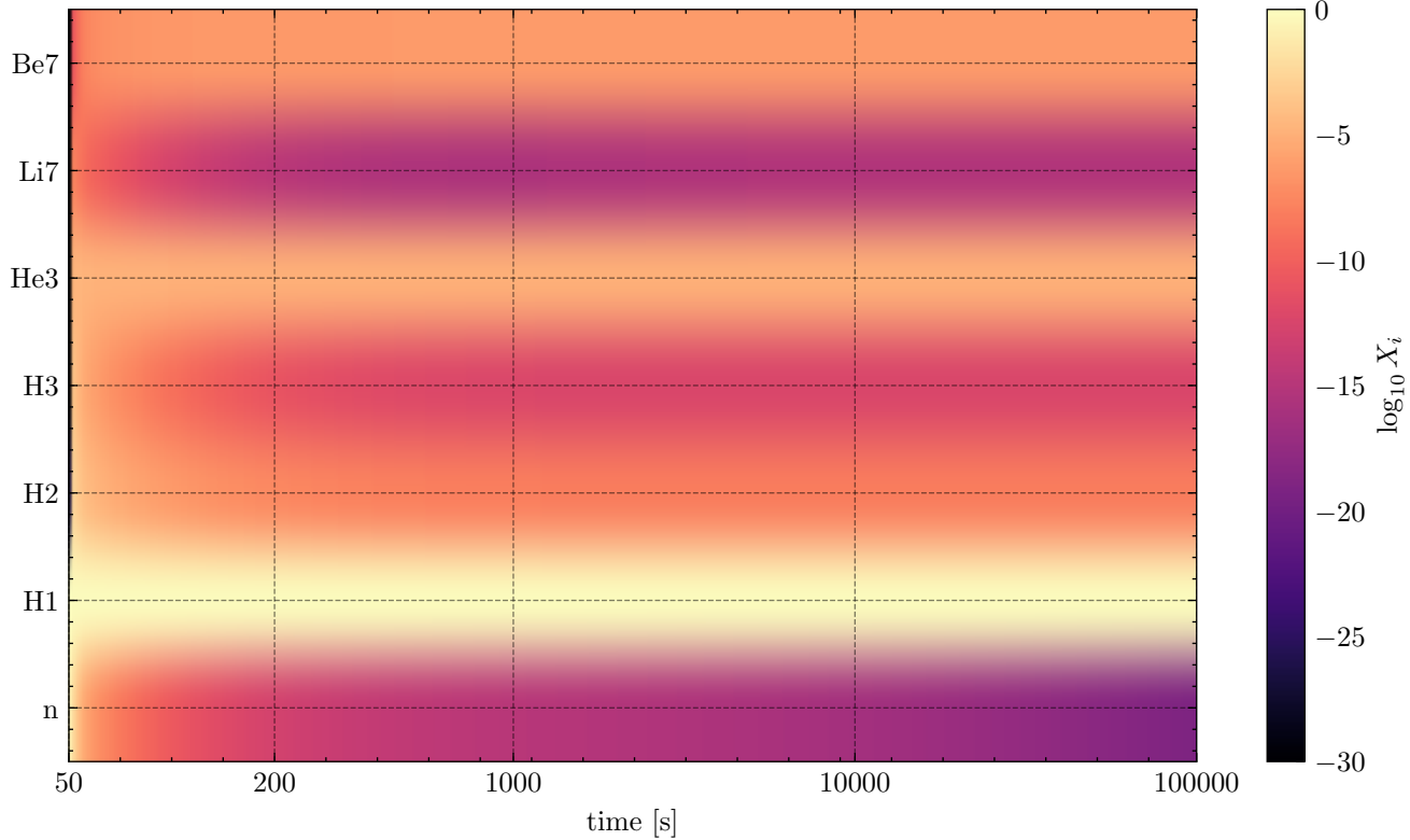
Abundance heatmap, t_0 = 50 s
