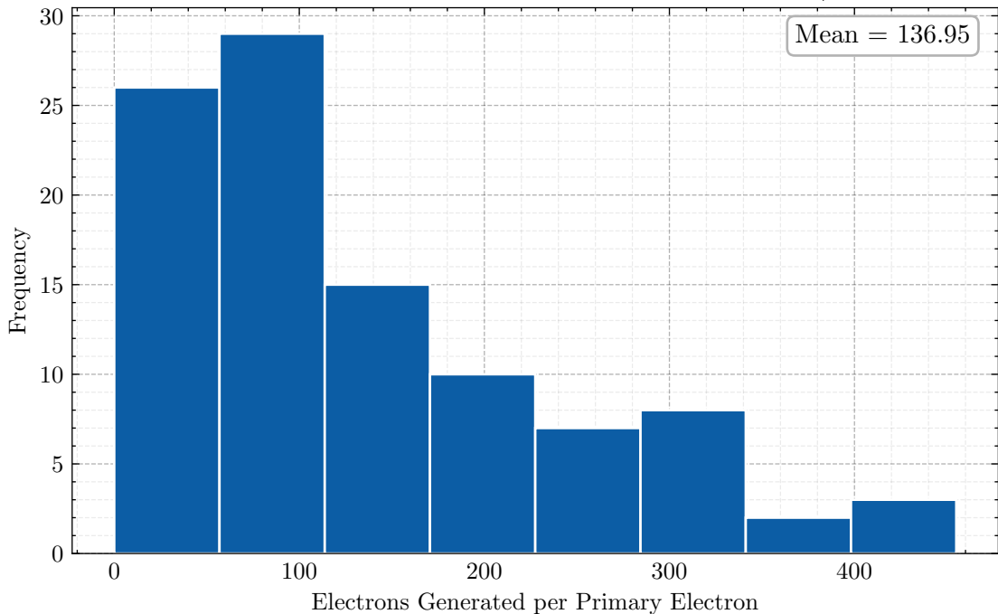
Electron Gain ar 99.0% - cf4 1.0% 0.05 bar 1.5 kV/cm
