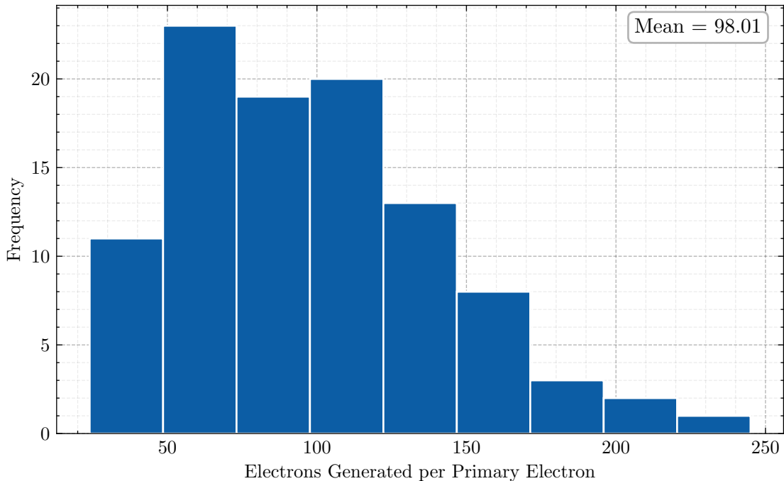
Electron Gain ar 99.5% - cf4 0.5% 0.2 bar 44.3 kV/cm
