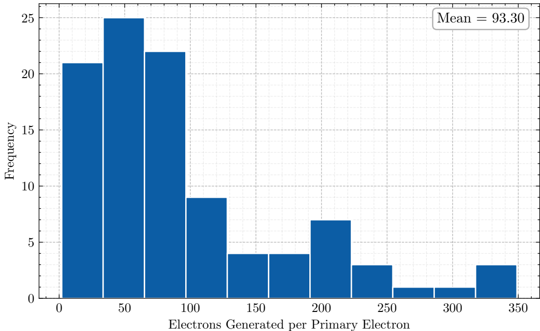
Electron Gain ar 99.8% - cf4 0.2% 1.0 bar 17.3 kV/cm
