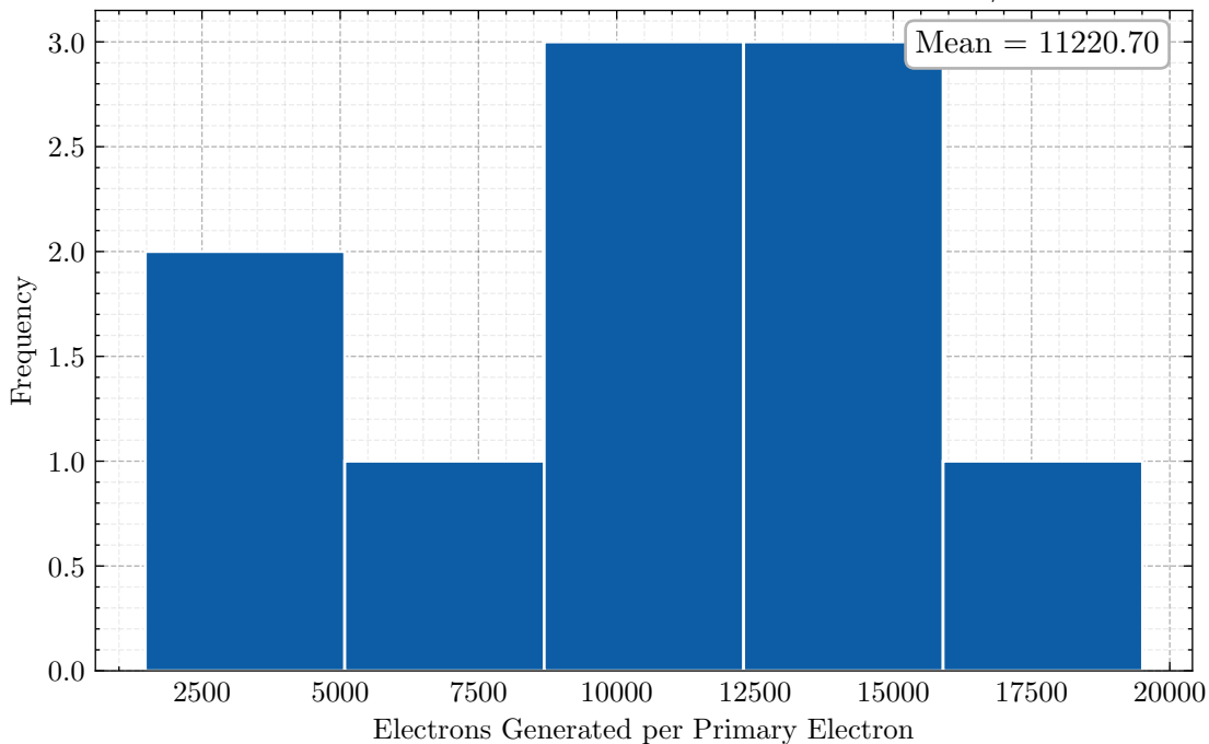
Electron Gain ar 99.0% - cf4 1.0% 1.0 bar 30.0 kV/cm
