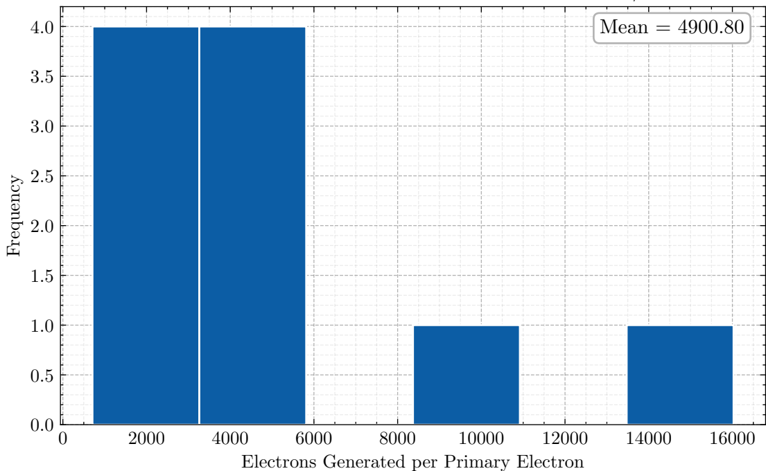
Electron Gain ar 99.0% - cf4 1.0% 1.0 bar 32.5 kV/cm
