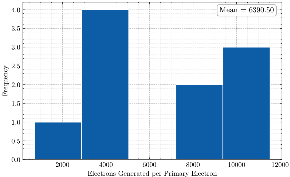
Electron Gain ar 99.0% - cf4 1.0% 1.0 bar 57.5 kV/cm
