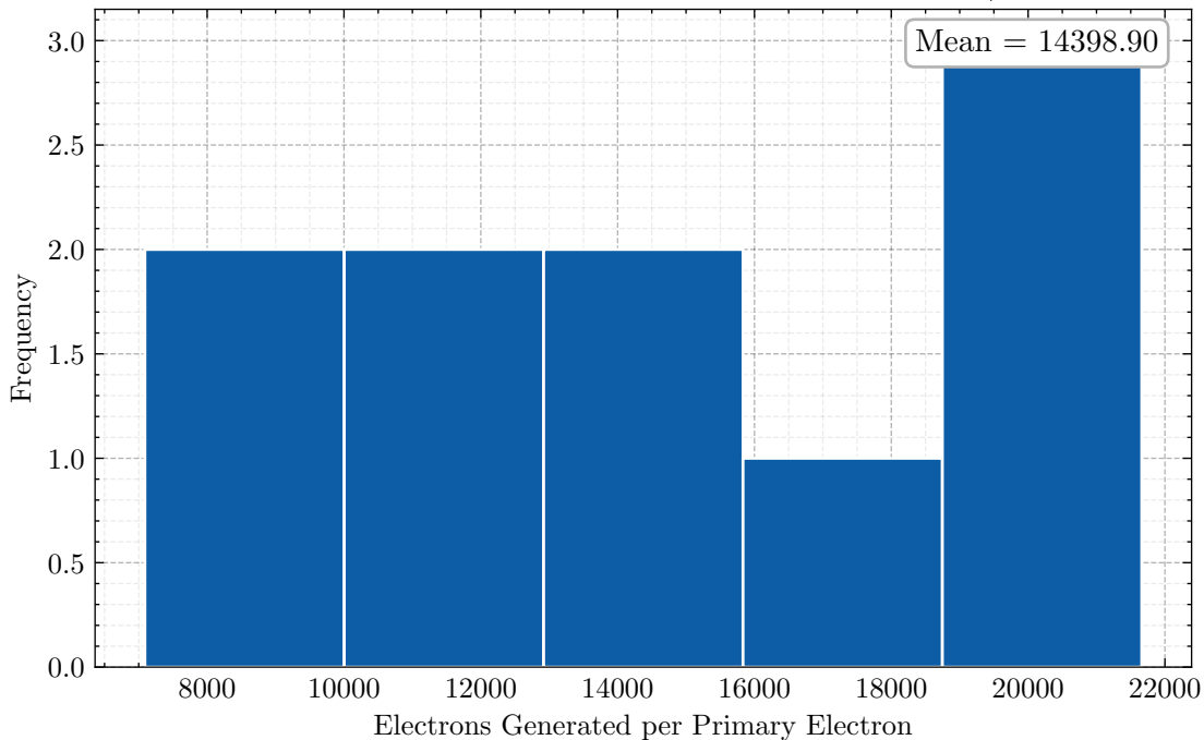
Electron Gain ar 99.0% - cf4 1.0% 1.0 bar 94.1 kV/cm
