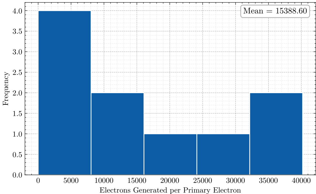
Electron Gain ar 99.5% - cf4 0.5% 10.0 bar 112.0 kV/cm
