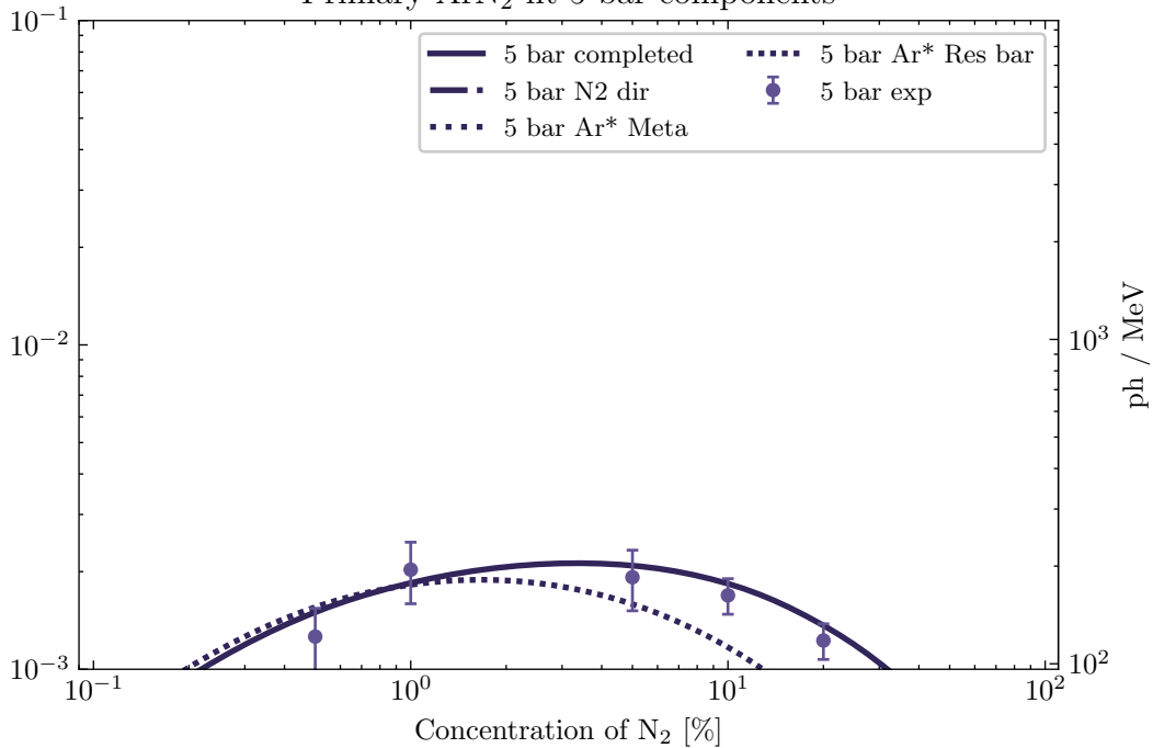
Primary ArN 2 fit 5 bar components
