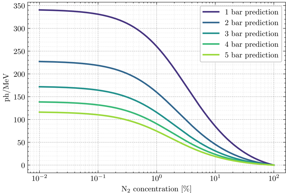
Primary ArN 2 IR (680-785nm) yield prediction
