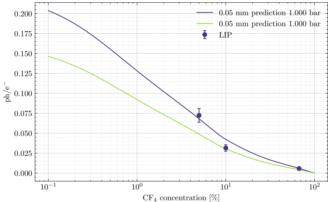
NIR (680-800nm) Yield Prediction for Ar/CF mixture
