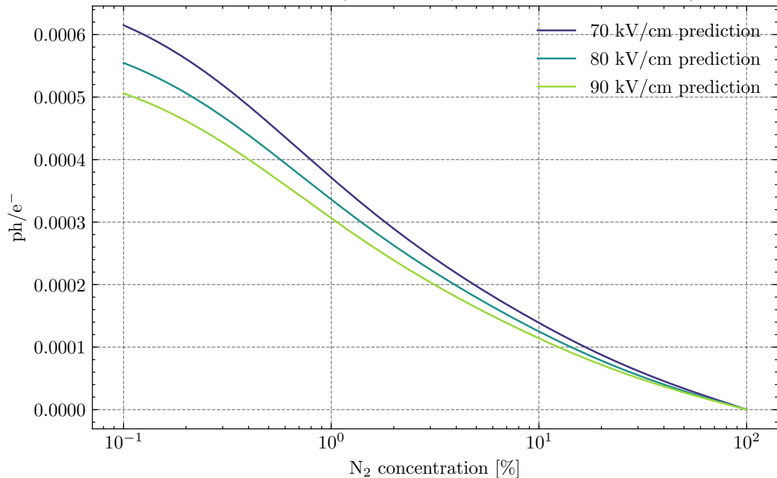
1 bar 10k gain secondary IR (680-785nm) Yield Prediction for Ar/N 2 mixture
